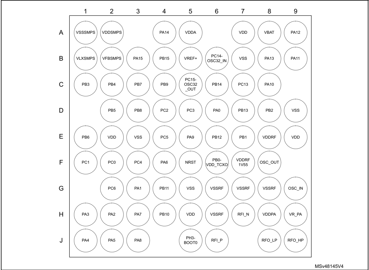
Figure 10. UFBGA73 pinout
