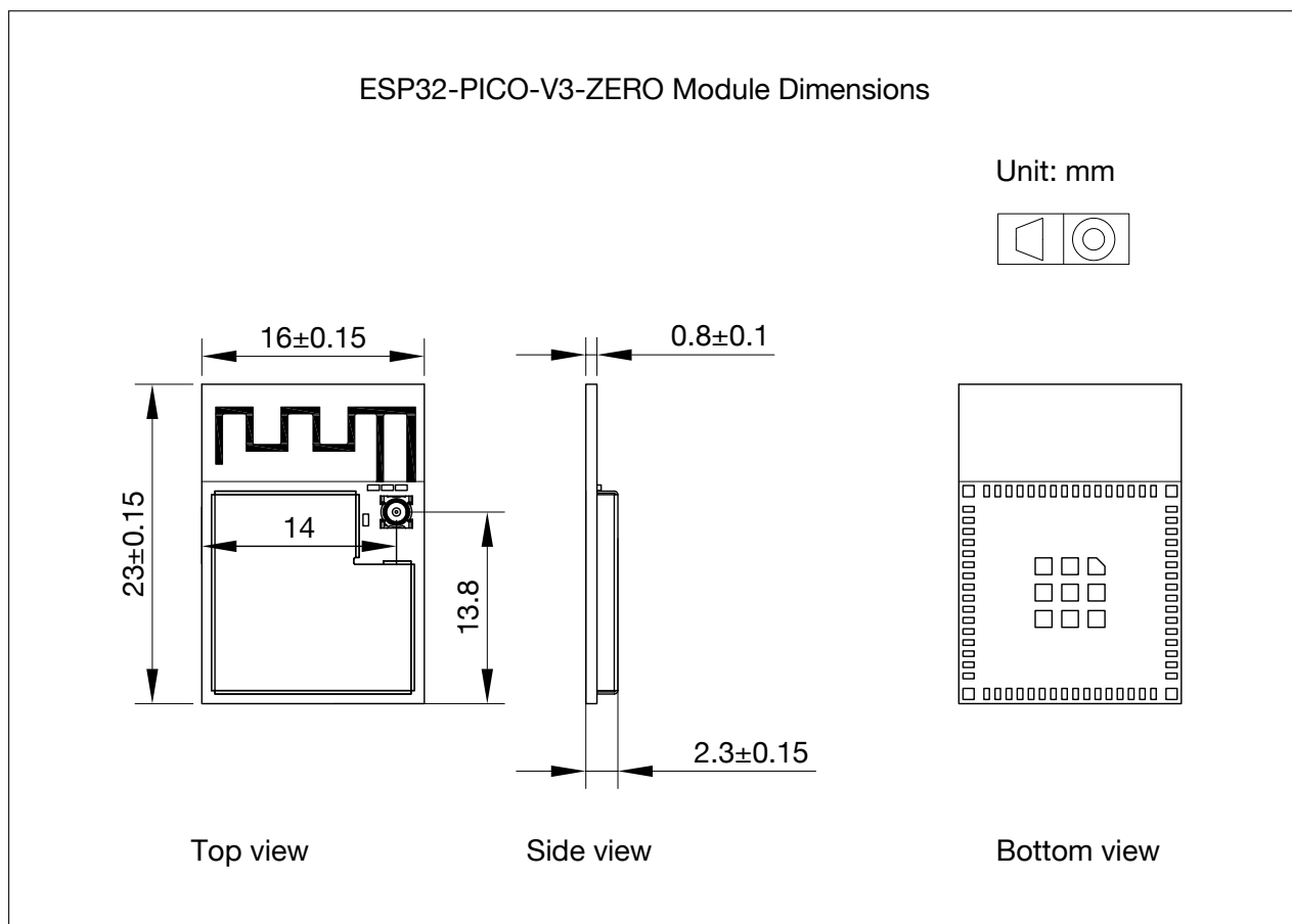
Figure 6: Physical Dimensions
