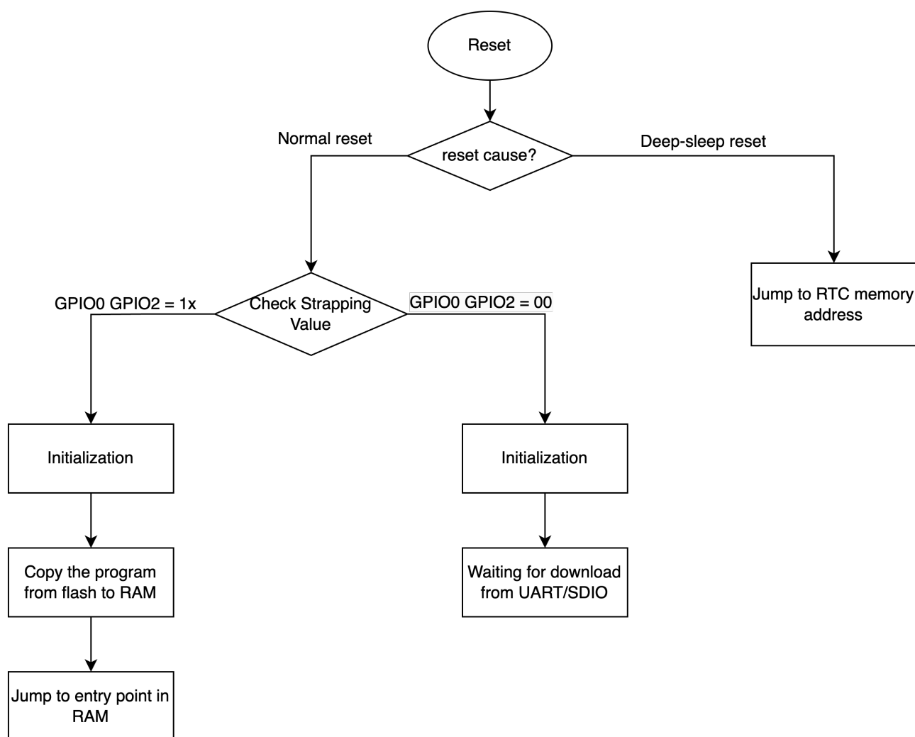
Figure 4: Chip Boot Flow
