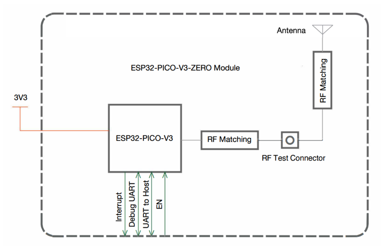
Figure 1: ESP32-PICO-V3-ZERO Block Diagram
