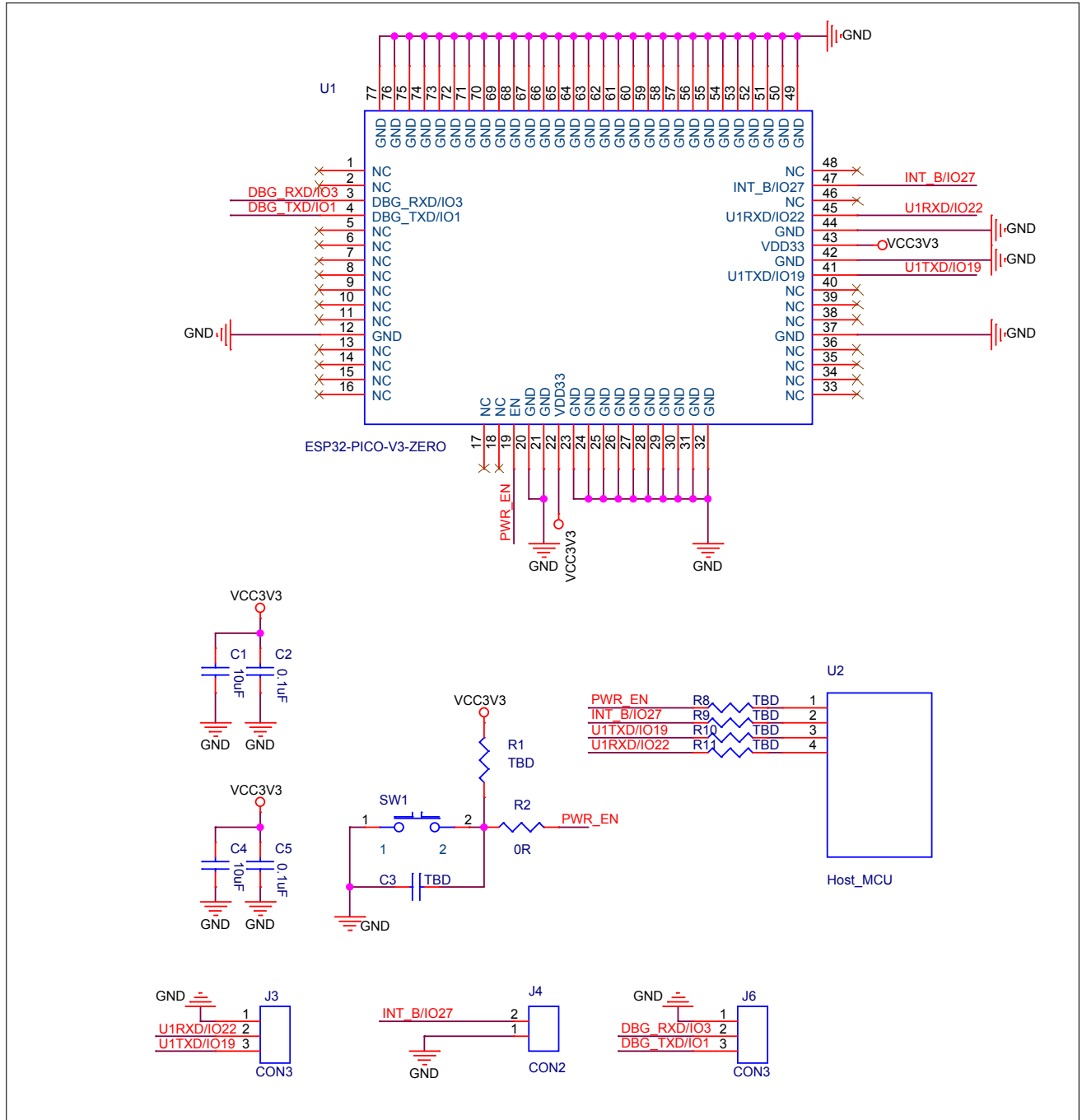
Figure 5: Peripheral Schematics
